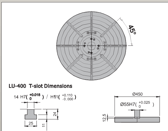
Worktable Dimension
