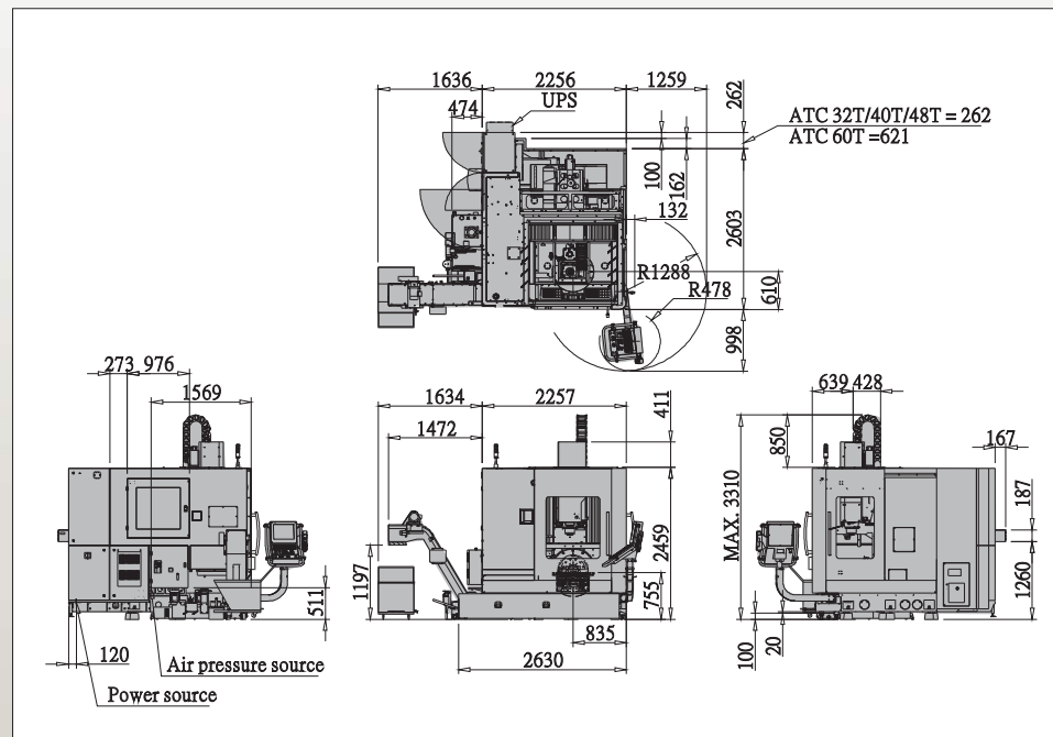
Appearance & Dimension
