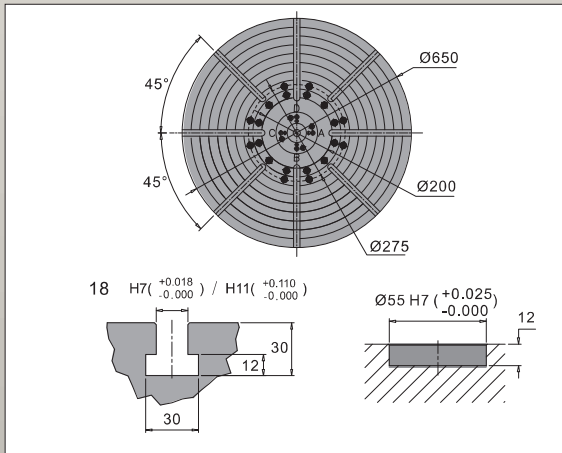
Worktable Dimension
