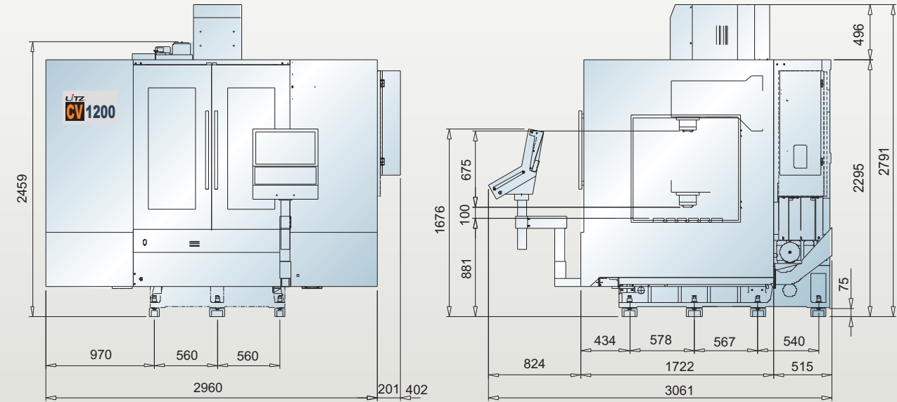
CV-1200
