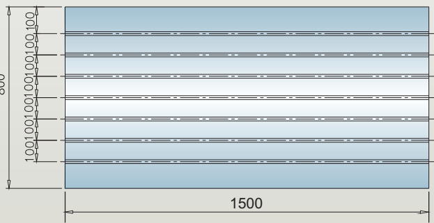
CV-1400N
