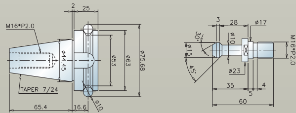
BT-40
