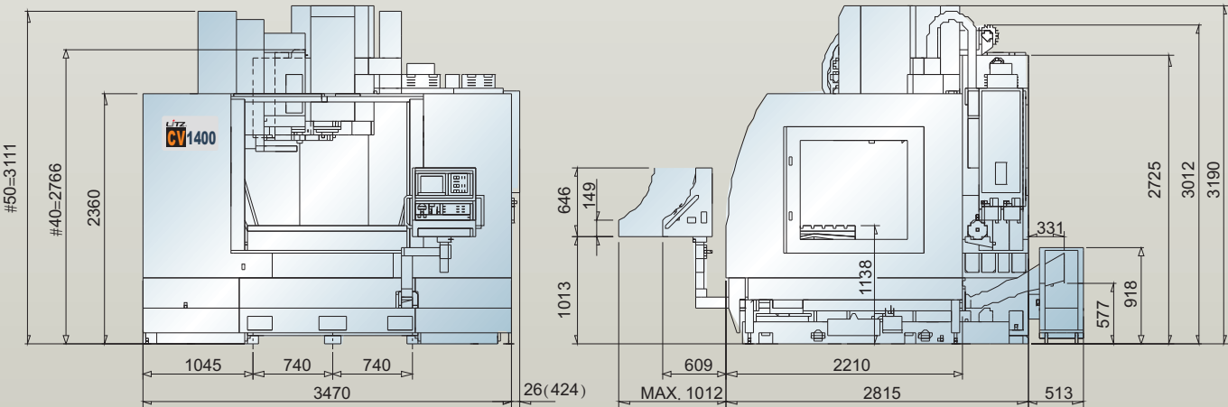
CV-1400N
