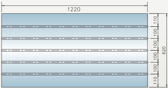
CV-1200
