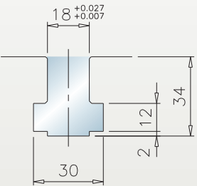
CV-1200 T-Slot dimensions
