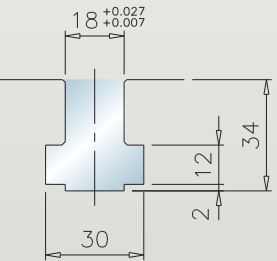
CV-1400N T-Slot dimensions
