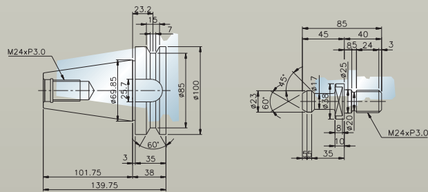
BT-50
