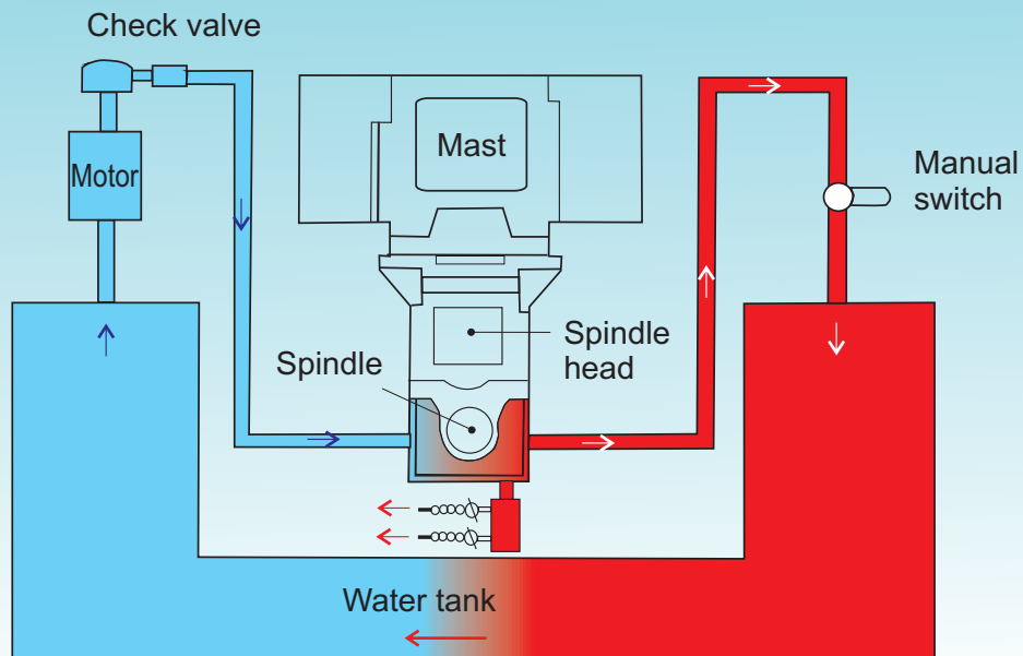
Spindle head water cooling diagram
