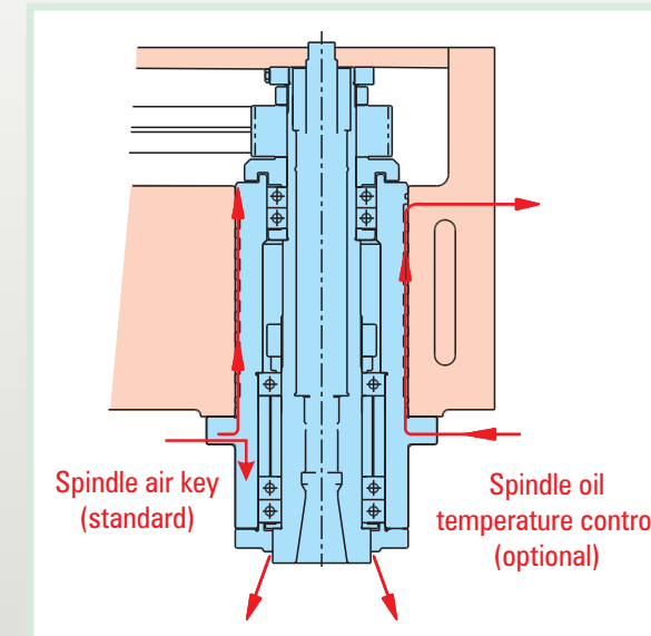
BT-40 spindle
