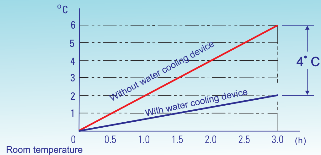
Spindle head water cooling benefits diagram
