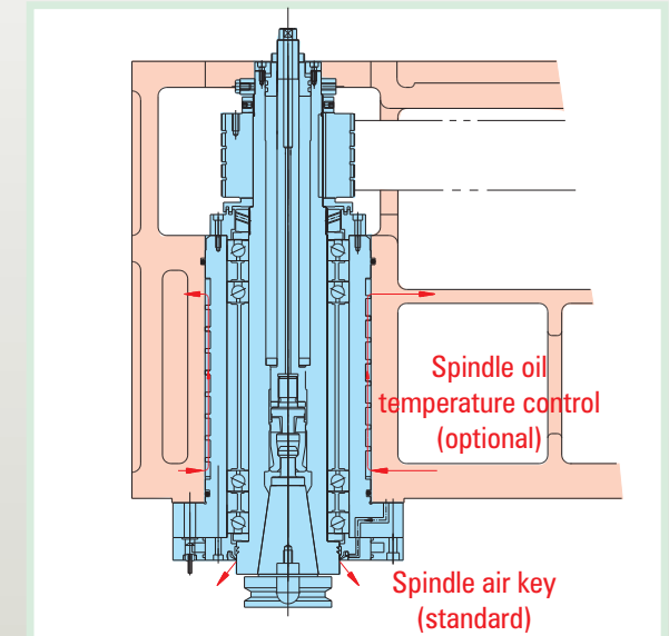
BT-50 spindle
