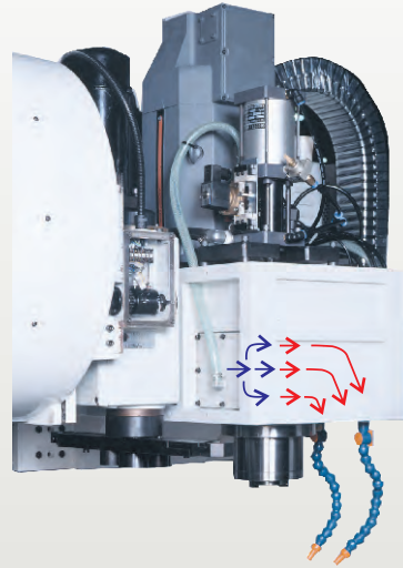
Spindle head water cooling diagram
