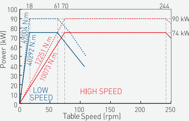
(MOTOR: FANUC \alpha il40/7000HVx2) High speed ratio: 16.40 Low speed ratio: 65.60 VTL1600ATC+C-2R Series
