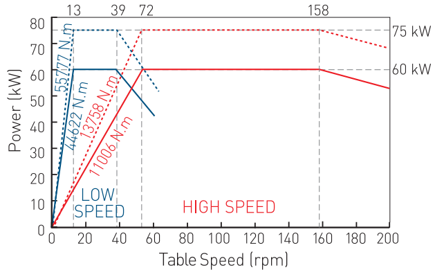
(MOTOR: FANUC \alpha il160/5000HV) High speed ratio: 22.10 Low speed ratio: 89.6 VTL2000ATC-2R Series
