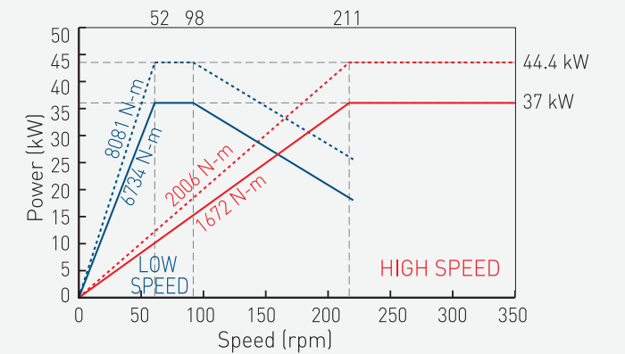
(MOTOR: SIEMENS 1PH8165-F) High speed ratio: 7.1 Low speed ratio: 28.6 VTL1200ATC+C Series
