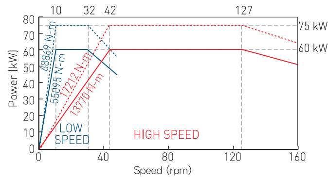
(MOTOR: FANUC αi160/5000HV) High speed ratio: 27.65 Low speed ratio: 110.63 VTL2500ATC Series
