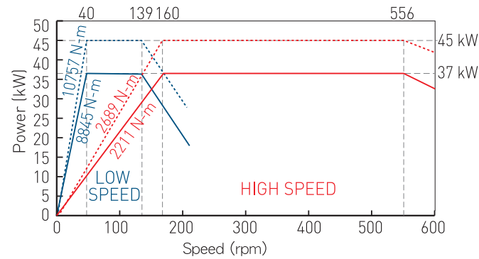
(MOTOR: FANUC αi140/7000) High speed ratio: 7.2 Low speed ratio: 28.8 VTL1000ATC Series
