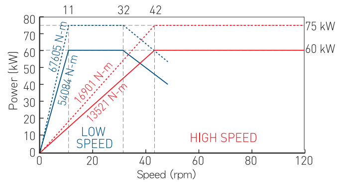
(MOTOR: FANUC αi160/5000HV) High speed ratio: 27.15 Low speed ratio: 108.60 VTL3000ATC Series
