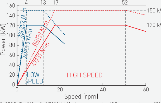
(MOTOR: FANUC \alpha il60/5000HVx2) High speed ratio: 67.5 Low speed ratio: 270.1 VTL3500ATC+C-2R Series
