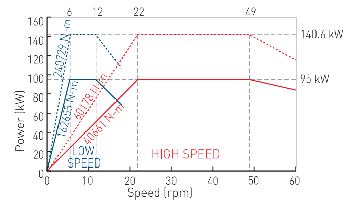
(MOTOR: SIEMENS 1PH8224-F) High speed ratio: 67.26 Low speed ratio: 269.06 VTL4000ATC/VTL4500ATC Series
