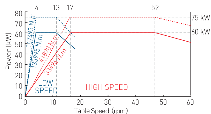
(MOTOR: FANUC αi160/5000HV) High speed ratio: 67.26 Low speed ratio: 269.06 VTL4000/4500ATC Series
