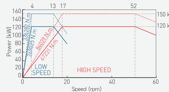
(MOTOR: FANUC αi160/5000HVx2) High speed ratio: 67.50 Low speed ratio: 270.10 VTL3500ATC+C Series
