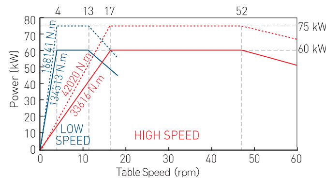
(MOTOR: FANUC αi160/5000HV) High speed ratio: 67.50 Low speed ratio: 270.10 VTL3500ATC Series
