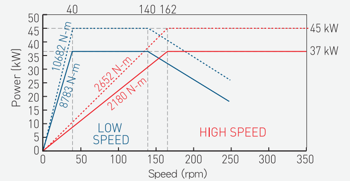
(MOTOR: FANUC αi140/7000) High speed ratio: 7.1 Low speed ratio: 28.6 VTL1200ATC+C Series
