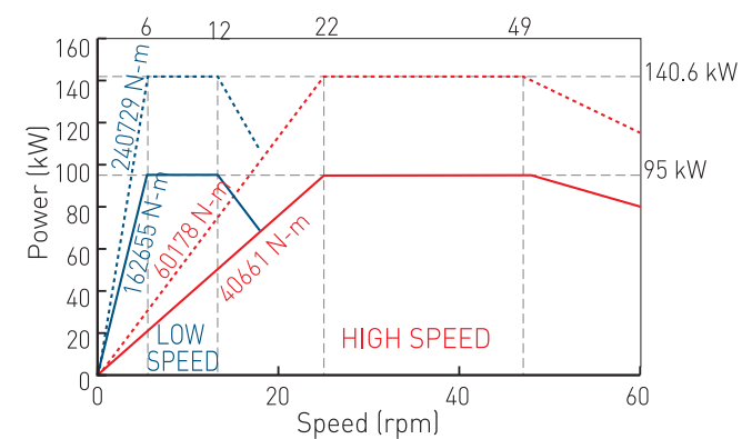
(MOTOR: SIEMENS 1PH8224-F) High speed ratio: 67.26 Low speed ratio: 269.06 VTL4000ATC-2R/VTL4500ATC-2R Series
