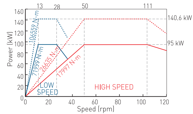
(MOTOR: SIEMENS 1PH8224-F) High speed ratio: 29.77 Low speed ratio: 119.1 VTL3000ATC-2R Series
