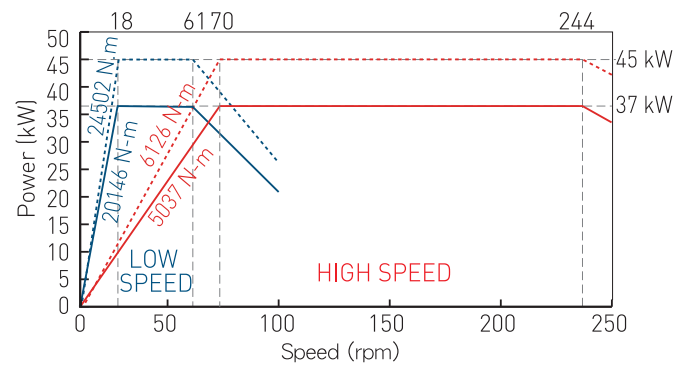
(MOTOR: FANUC αi140/7000) High speed ratio: 16.4 Low speed ratio: 65.6 VTL1600ATC Series
