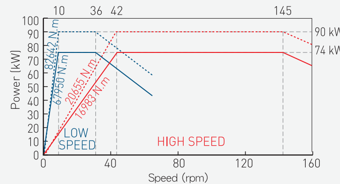
(MOTOR: FANUC αi140/7000HVx2) High speed ratio: 27.65 Low speed ratio: 110.63 VTL2500ATC+C Series (Opt.)
