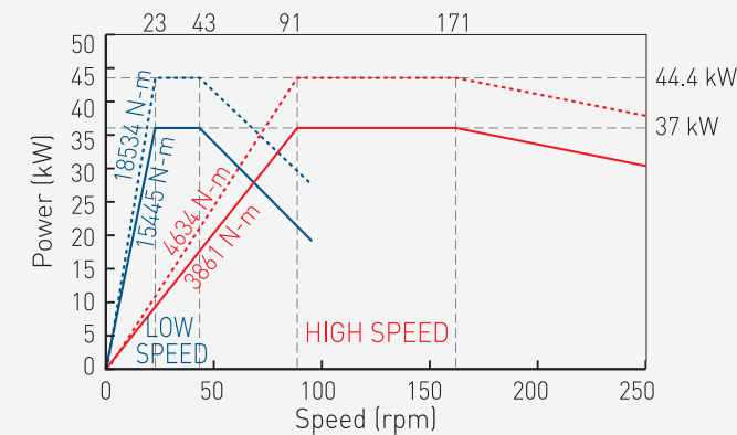
(MOTOR: SIEMENS 1PH8165-F) High speed ratio: 16.4 Low speed ratio: 65.6 VTL1600ATC+C Series
