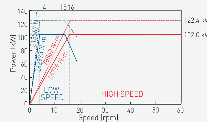
(MOTOR: SIEMENS 1PH8186-Dx2) High speed ratio: 67.5 Low speed ratio: 270.1 VTL3500ATC+C Series
