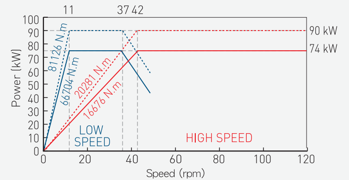
(MOTOR: FANUC αi140/7000HVx2) High speed ratio: 27.15 Low speed ratio: 108.60 VTL3000ATC+C Series
