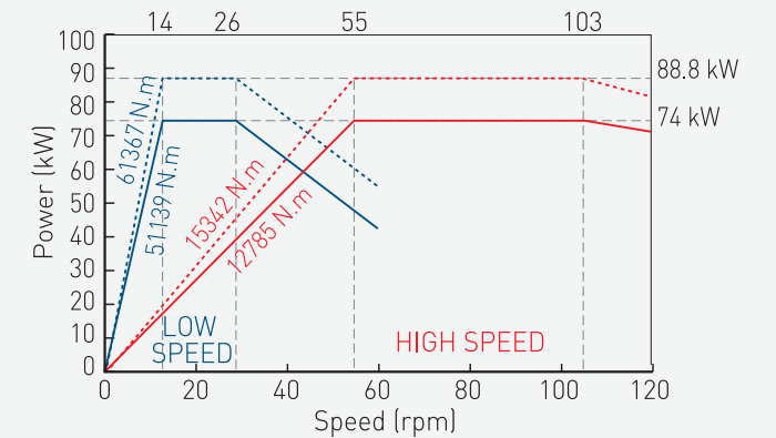
(MOTOR: SIEMENS 1PH8165-Fx2) High speed ratio: 27.15 Low speed ratio: 108.6 VTL3000ATC+C Series
