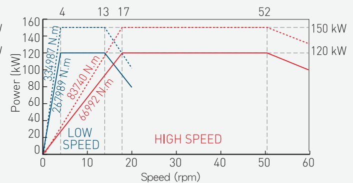
(MOTOR: FANUC αi160/5000HVx2) High speed ratio: 67.26 Low speed ratio: 269.06 VTL4000ATC+C/VTL4500ATC+C Series
