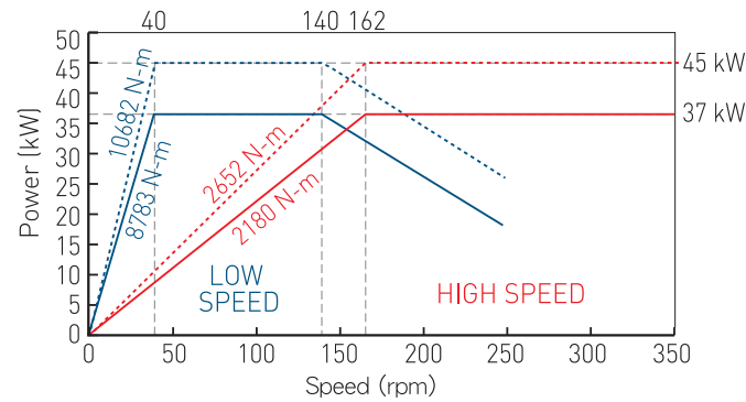
(MOTOR: FANUC αi140/7000) High speed ratio: 7.1 Low speed ratio: 28.6 VTL1200ATC Series
