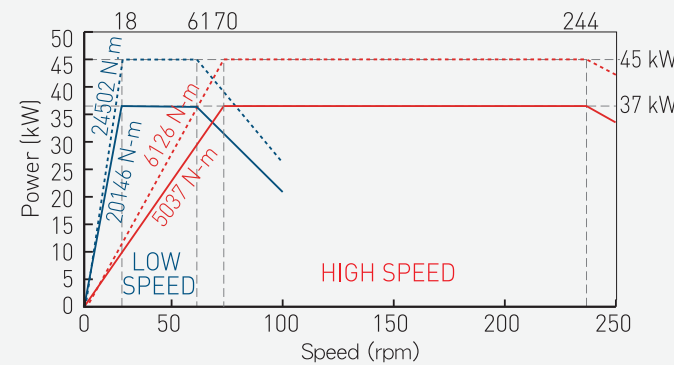
(MOTOR: FANUC αi140/7000) High speed ratio: 16.4 Low speed ratio: 65.6 VTL1600ATC+C Series
