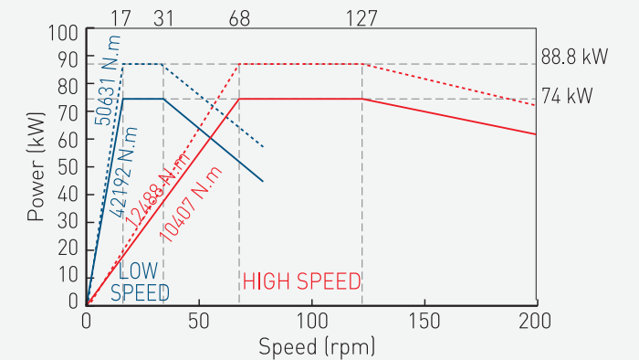
(MOTOR: SIEMENS 1PH8165-Fx2) High speed ratio: 22.1 Low speed ratio: 89.6 VTL2000ATC+C Series (Opt.)
