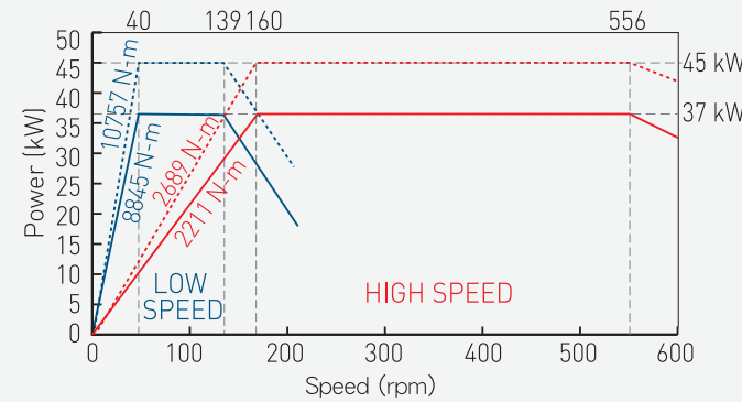
(MOTOR: FANUC αi140/7000) High speed ratio: 7.2 Low speed ratio: 28.8 VTL1000ATC+C Series
