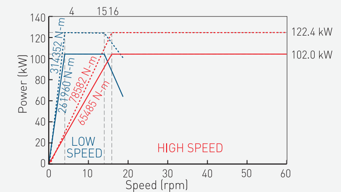
(MOTOR: SIEMENS 1PH8186-Dx2) High speed ratio: 67.26 Low speed ratio: 269.06 VTL4000ATC+C/VTL4500ATC+C Series
