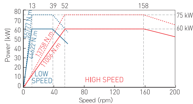
(MOTOR: FANUC αi160/5000HV) High speed ratio: 22.1 Low speed ratio: 89.6 VTL2000ATC Series
