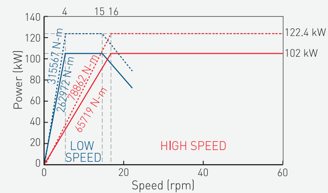
(MOTOR: SIEMENS 1PH8186-Dx2) High speed ratio: 67.50 Low speed ratio: 270.1 VTL3500ATC+C-2R Series
