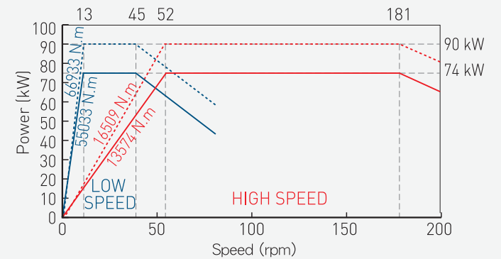
(MOTOR: FANUC αi140/7000HVx2) High speed ratio: 22.1 Low speed ratio: 89.6 VTL2000ATC+C Series (Opt.)
