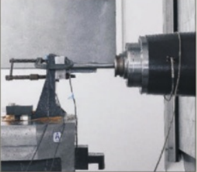
On-line Measurement System
