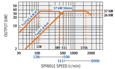
Main spindle power-torque diagram
