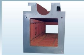
●立柱 床台皆採堅固的箱型結構，鑄件內部 配置強化肋骨，且配合FC-30 米漢納 材質，並經淬火調質處理，無變型之 慮，極具強剛性。 The bed and column are designed as box type with rigid structures. All the main components are made of FC-30 high quality casting and annealing heat treatment.
