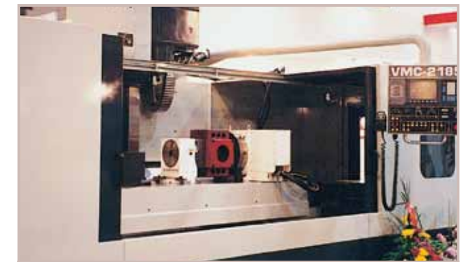
NCF-400 + TSA-251S (Special tailstock + 4 faces fixture plate) Application : Vertical / Horizontal Machining Center
